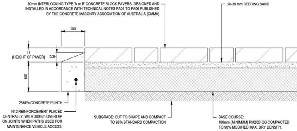
SECTION THROUGH EDGE OF FOOTPATH SCALE 1:5
